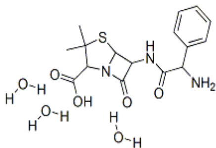
Figure 1: Structure of Ampicillin.
