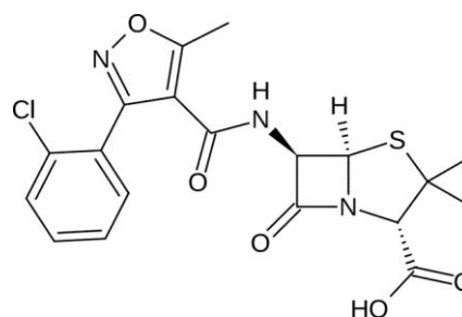
Figure 2: Structure of Cloxacillin.
