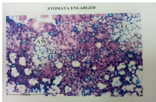
Fig. 9: Stomata enlarged.
