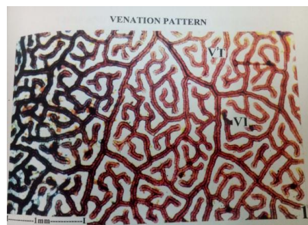
Fig. 10: Venation pattern.
