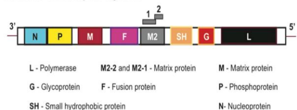
Figure 1: A simplified illustration of HMPV structure showing key proteins (N, M, G, F).
