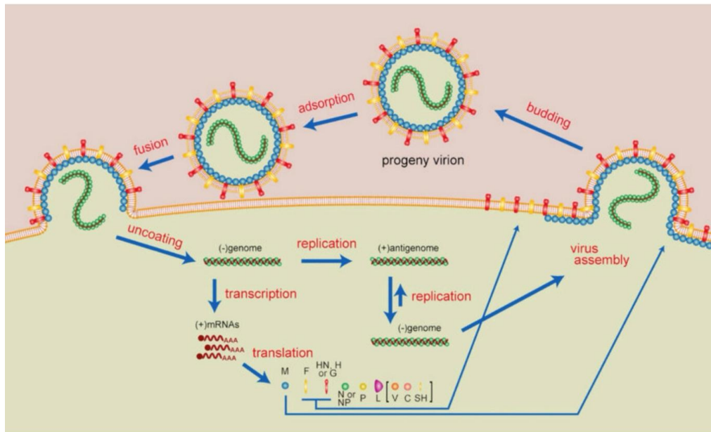
Schematic illustration of a paramyxovirus life cycle
